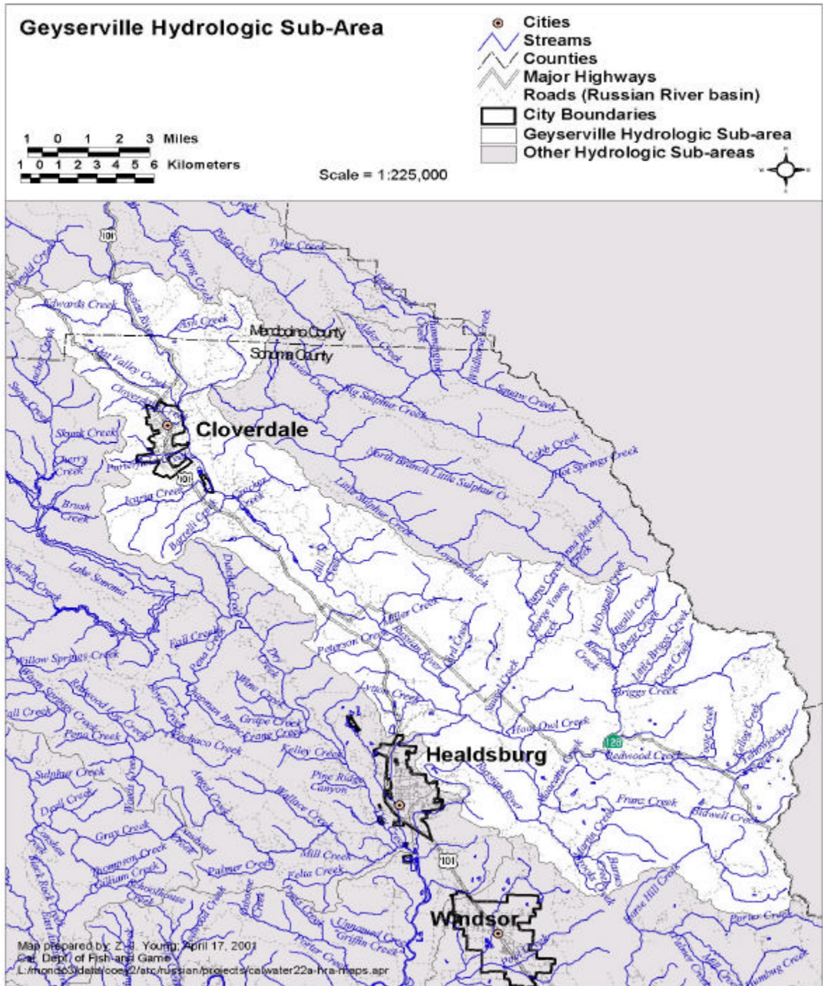
Figure 23. Geyserville hydrologic sub-area.
