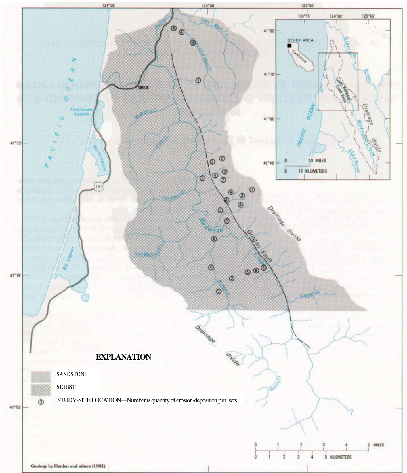
FIGURE 1.—Major bedrock types and study-site locations.
