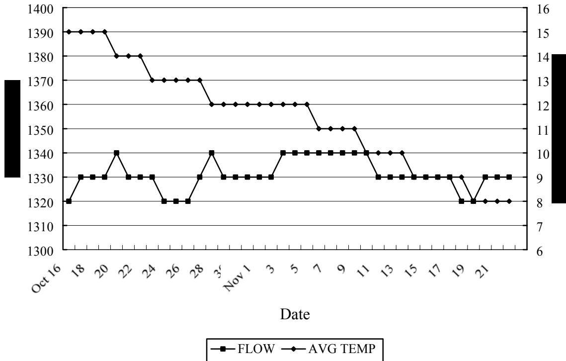
Figure 9. Water temperatures (C) at rkm 300.4 and discharge from Iron Gate Dam (October 16 to November 22).
