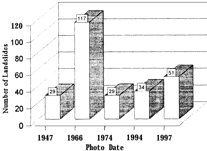
Figure 4. Landslide Frequency
